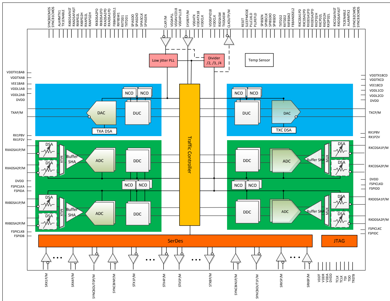
Figure 1-2. Functional Block Diagram of AFE7684
