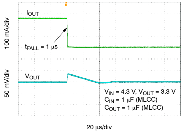
Figure 33. Load Transient Response – 250 mA to 1 mA – V_{OUT} = 3.3\text{ V}
