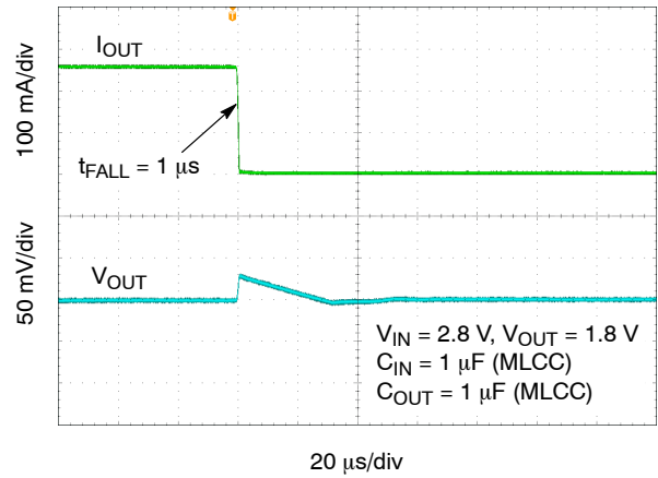
Figure 31. Load Transient Response – 250 mA to 1 mA – V_{OUT} = 1.8\text{ V}
