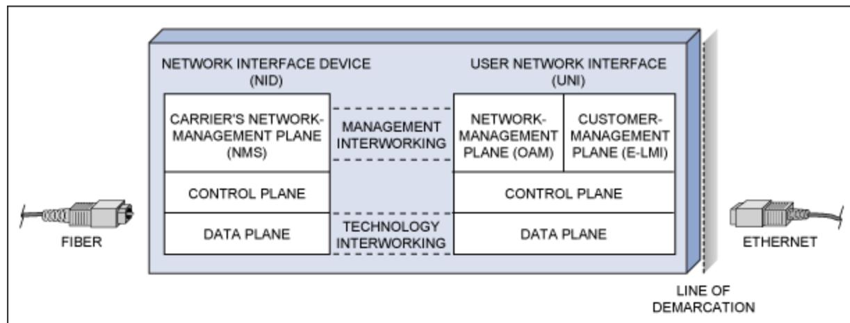
Figure 1. A functional block diagram is shown for an Ethernet demarcation unit. UNI comprises the
