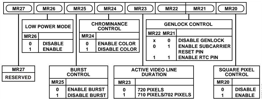
Figure 40. Mode Register 2
