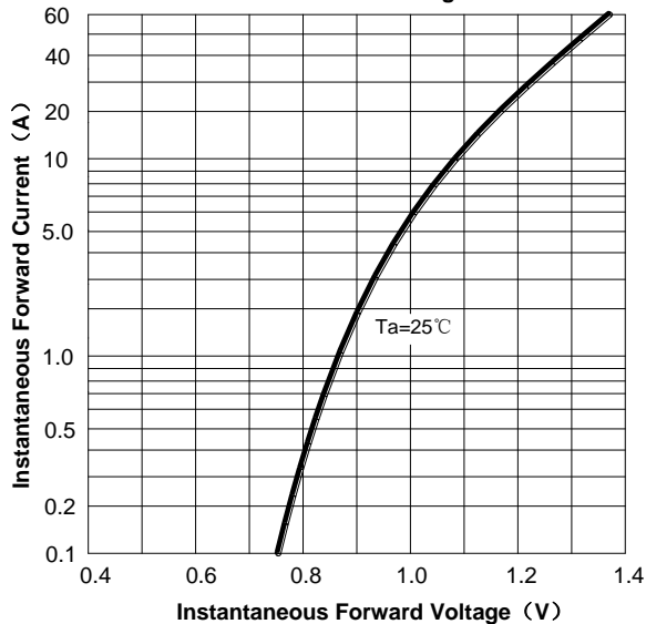
FIG3: Forward Voltage
