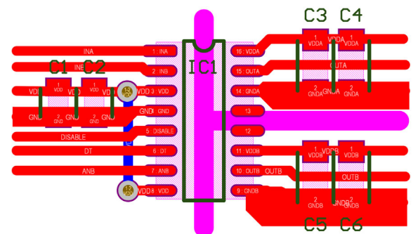
Figure 15. Recommended Layout (NCx57255, NCx57256)
